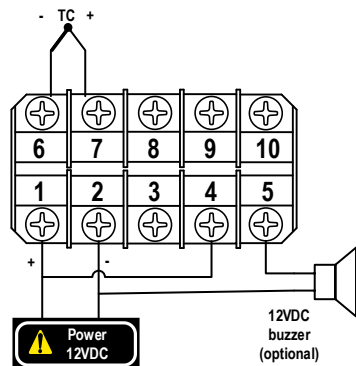
Figure 6. Wiring SYL-1813 with an EGT probe and an alarm buzzer.
