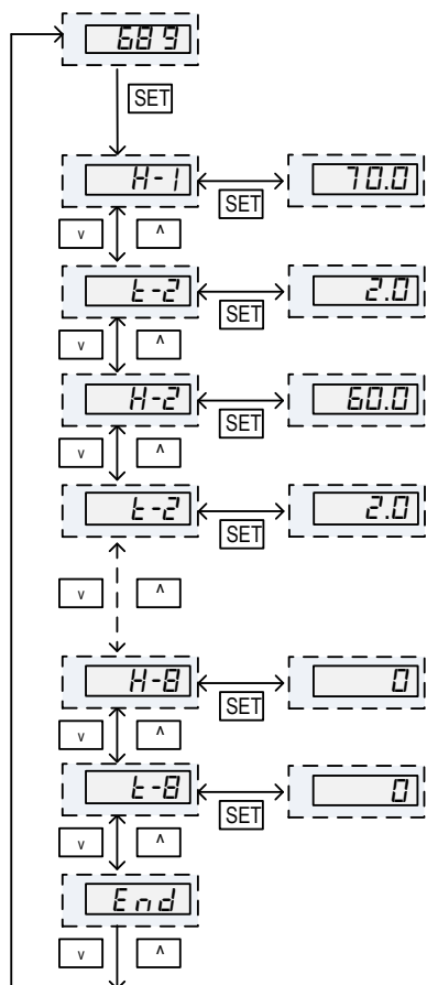
Figure 4. Flow chart of setting up control program.
