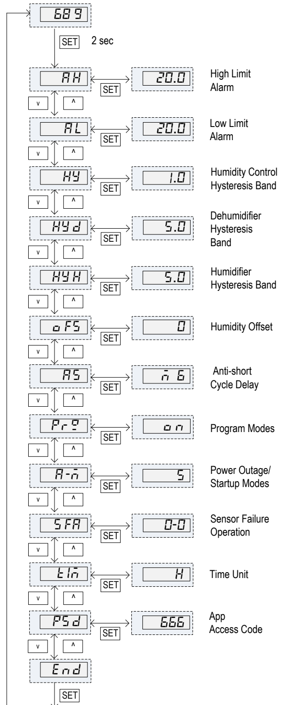
Figure 3. Flow chart of setting up parameters.
