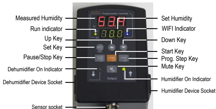
Figure 1. Front Panel.
