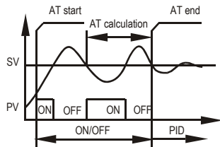
Figure 8. Auto tuning
